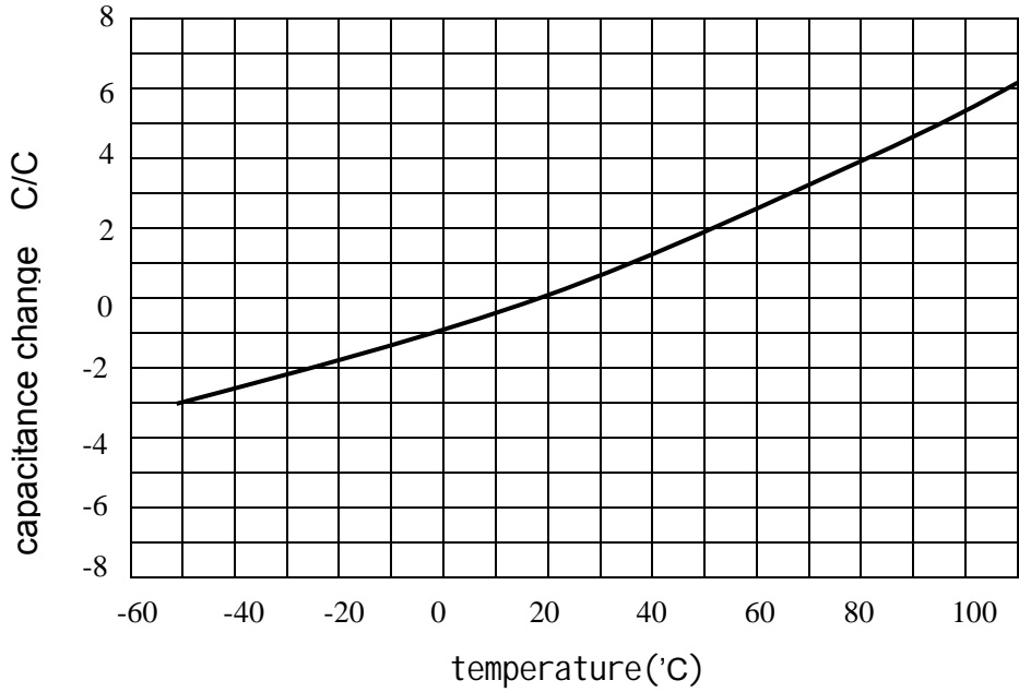
9.2 capacitance change vs temperature
