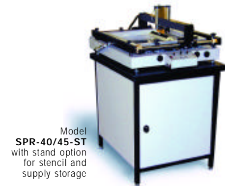
Model SPR-45 semi-automatic stencil printer
