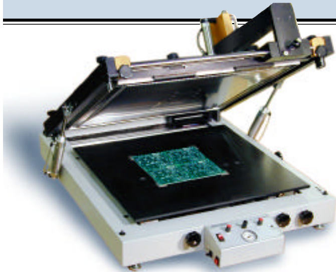
Model SPR-45 semi-automatic stencil printer
